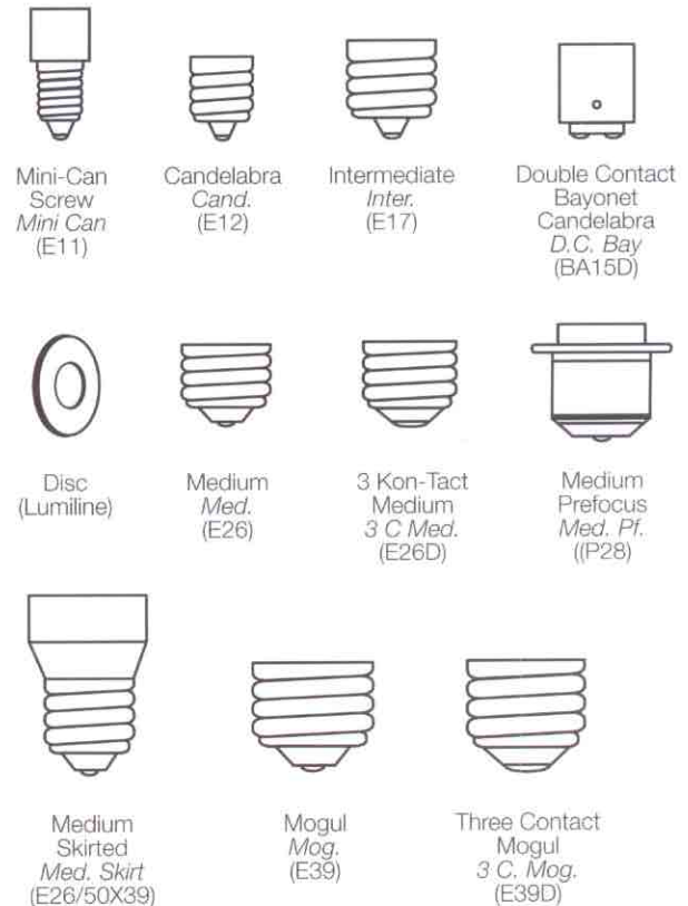
Figure 8. Typical Lamp Bases
