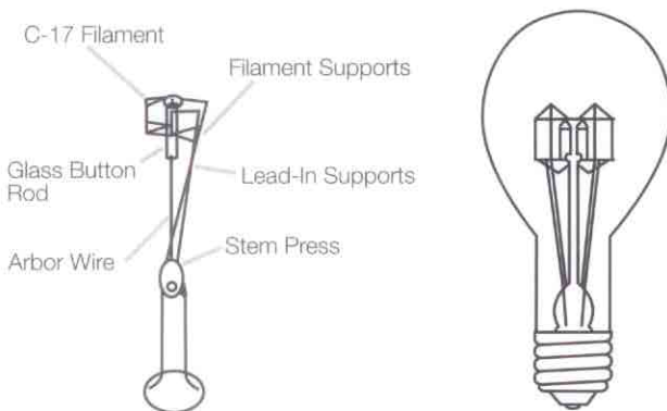
Figure 9. Typical Rough Service Lamp
