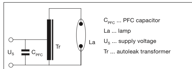
Fig. 7: Autoleak transformer
