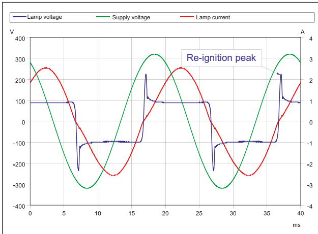
Fig. 30: Re-ignition peak, supply voltage and lamp current
