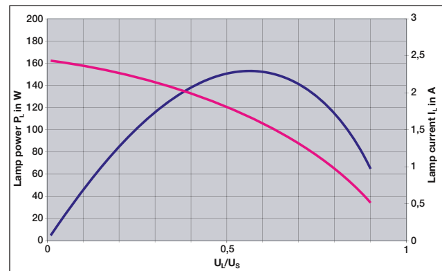
Fig. 10: Lamp current I_L , lamp wattage P_L over the ratio of lamp voltage to supply voltage U_L/U_s at U_N=200 V
