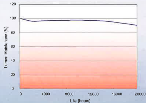
LUMEN MAINTENANCE
