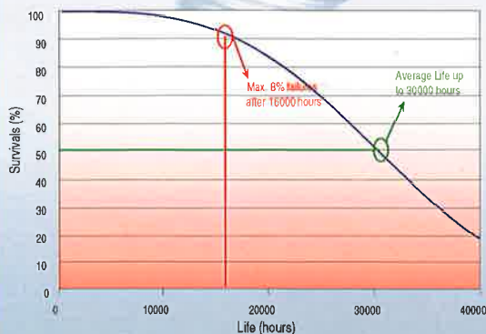
SURVIVAL CURVE
