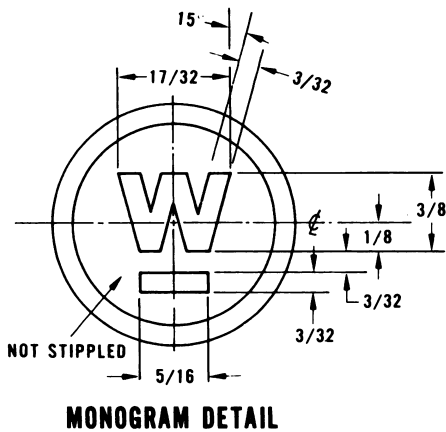
FIGURE 3b. Additional Westinghouse logo details. Center monogram used on Westinghouse 6006 and 6012 lamps from February 1968 to present. Center monogram used on Westinghouse 4001 and 4002 lamps from 1956 to April 1962.
