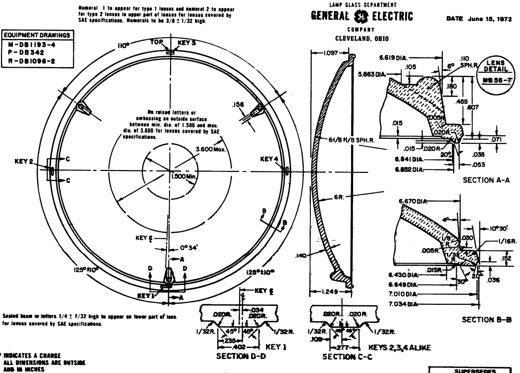
FIGURE C16. G.E. PAR 56 lamp lens detail. This modifies specifications in figure C15.
