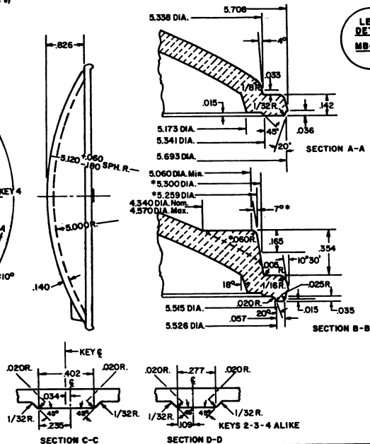
FIGURE C8. General Electric PAR 46 lamp lens detail.
