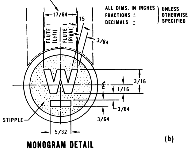
FIGURE 3b. Additional Westinghouse logo details. Center monogram used on Westinghouse 6006 and 6012 lamps from February 1968 to present. Center monogram used on Westinghouse 4001 and 4002 lamps from 1956 to April 1962.
