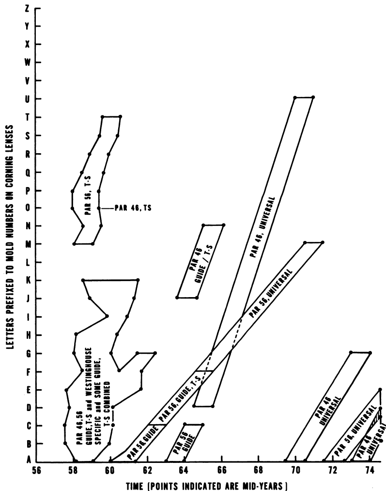
FIGURE 5. Time distributions for the alphabetic prefixes to Corning's PAR 46 and PAR 56 lens molds numbers (based on the data in table 10).
