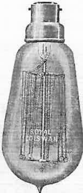
200-260 Volts. Cone Shape. 52-63 Watts.
